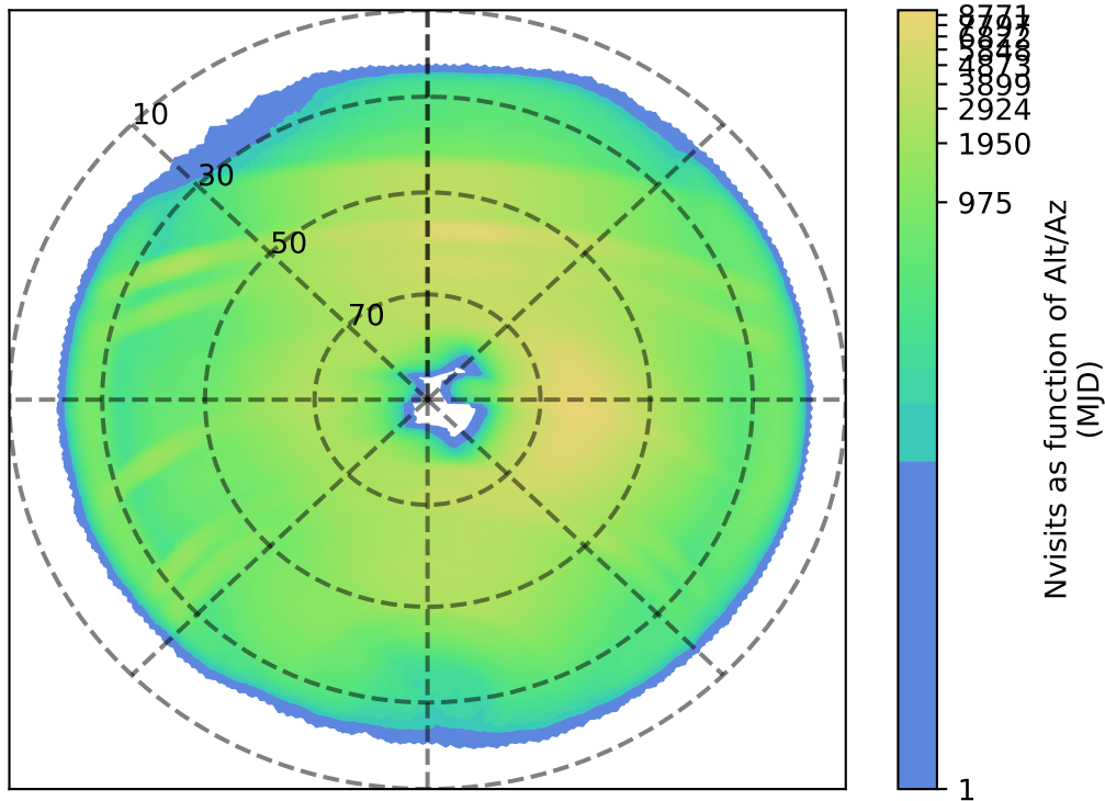
baseline_v3.3_10yrs : Nvisits as function of Alt/Az
