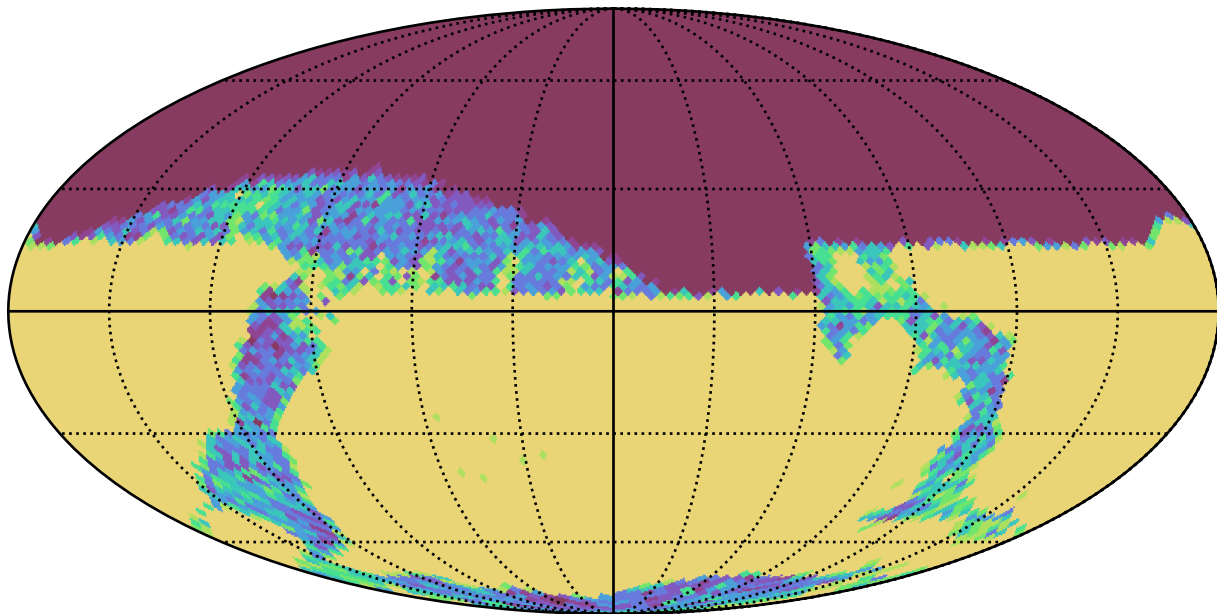
baseline_v3.3_10yrs z and night < 365: N year 1
