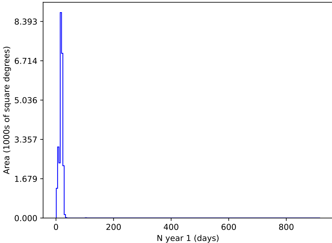
baseline_v3.3_10yrs y and night < 365: N year 1
