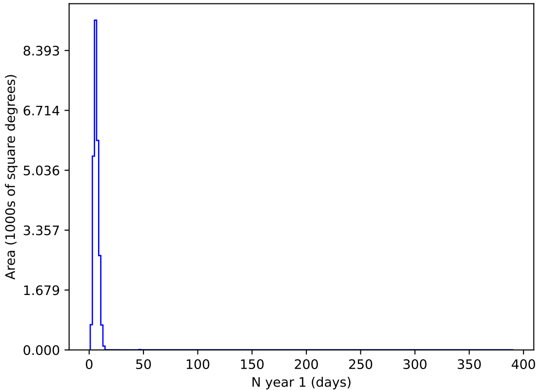
baseline_v3.3_10yrs u and night < 365: N year 1
