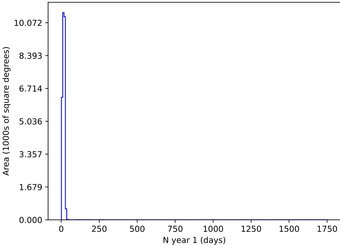
baseline_v3.3_10yrs r and night < 365: N year 1
