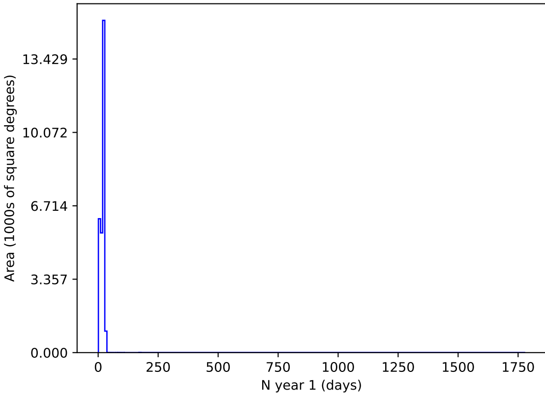
baseline_v3.3_10yrs i and night < 365: N year 1
