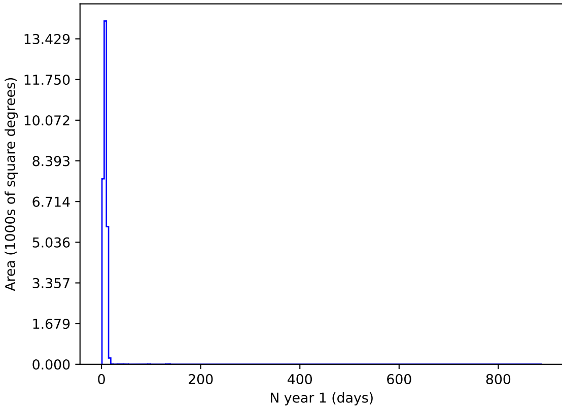
baseline_v3.3_10yrs g and night < 365: N year 1
