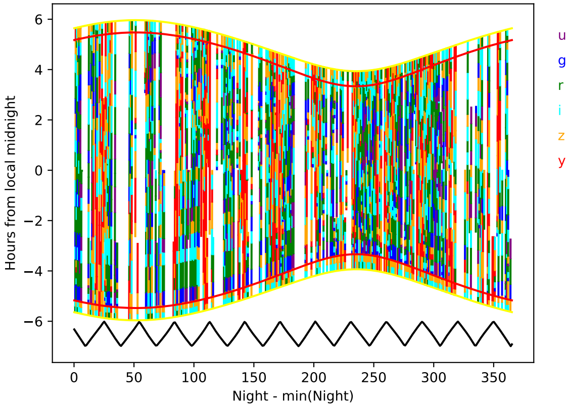
baseline_v3.3_10yrs year 7-8: Hourglass
