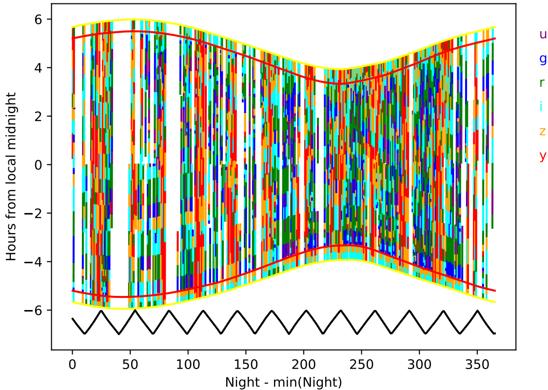
baseline_v3.3_10yrs year 4-5: Hourglass
