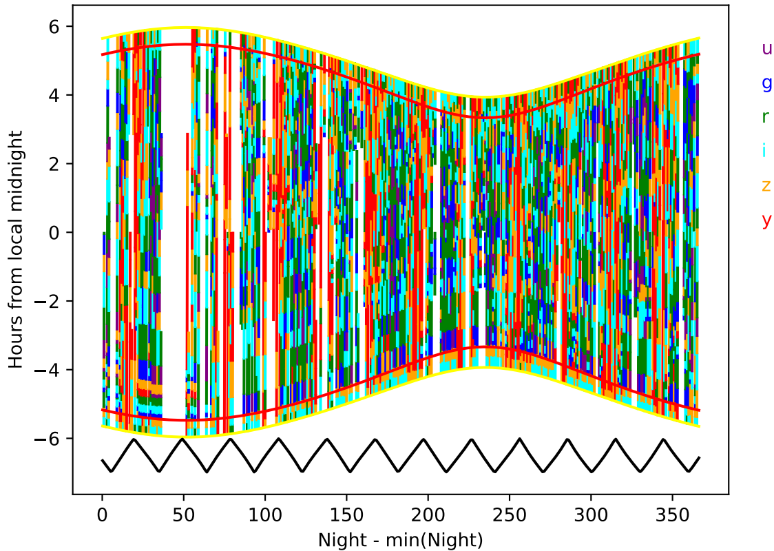
baseline_v3.3_10yrs year 2-3: Hourglass
