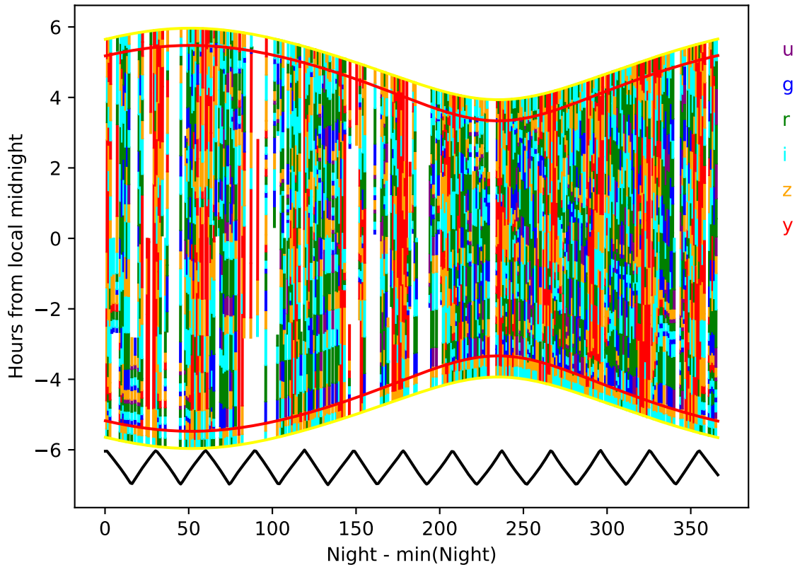
baseline_v3.3_10yrs year 1-2: Hourglass
