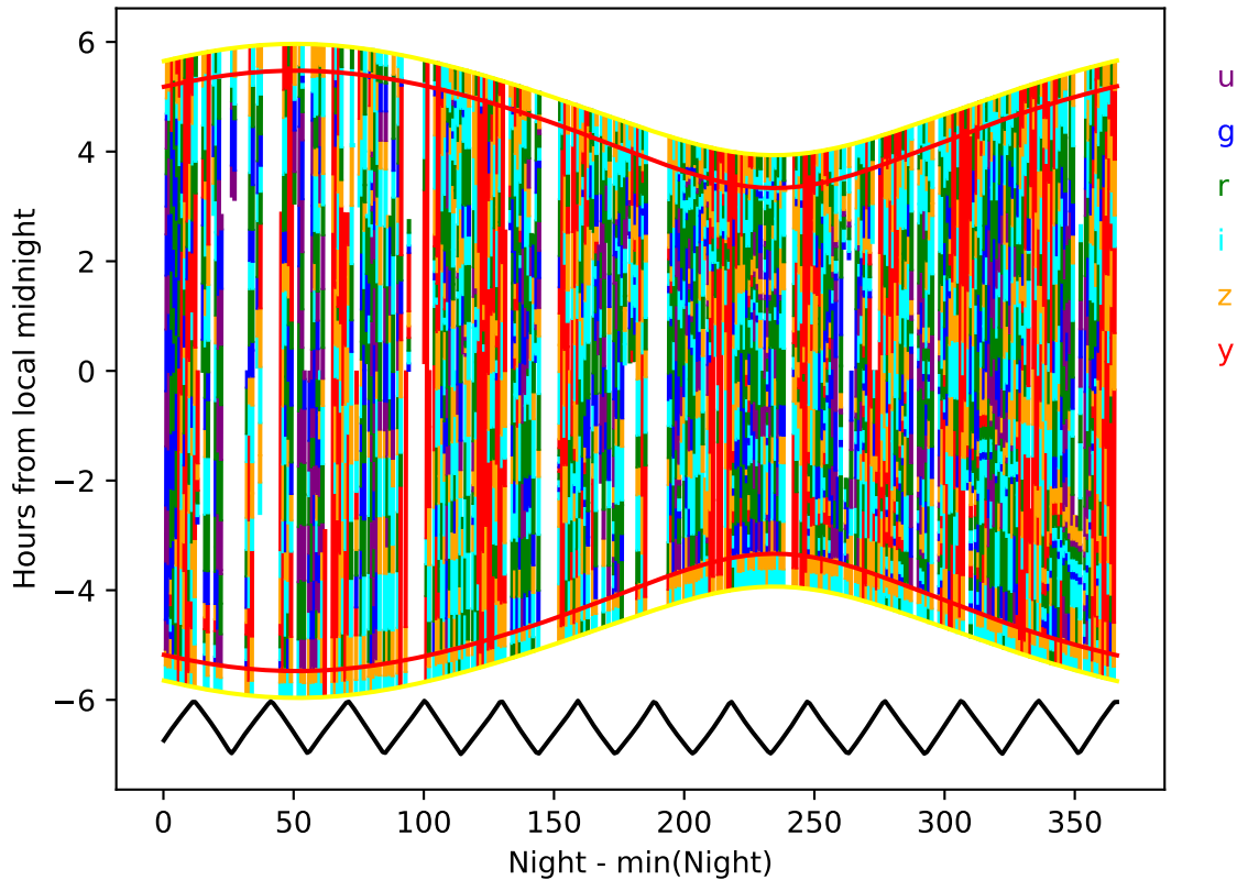
baseline_v3.3_10yrs year 0-1: Hourglass
