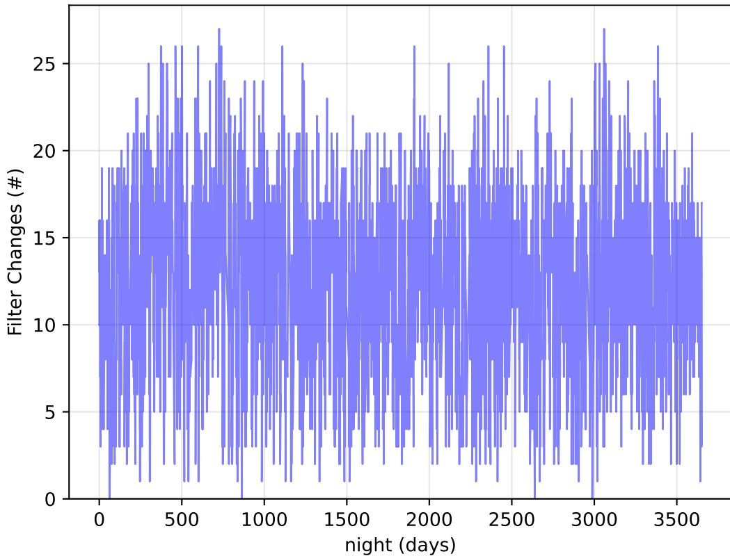
baseline_v3.3_10yrs : Filter Changes
