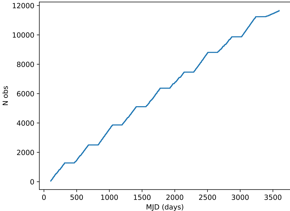
baseline_v3.3_10yrs note like DD:EDFS_a%: Cumulative
