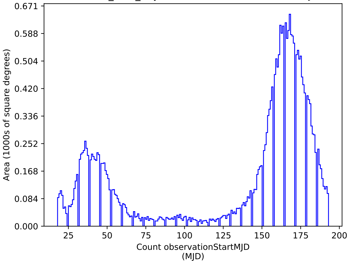
baseline_v3.3_10yrs z: Count observationStartMJD
