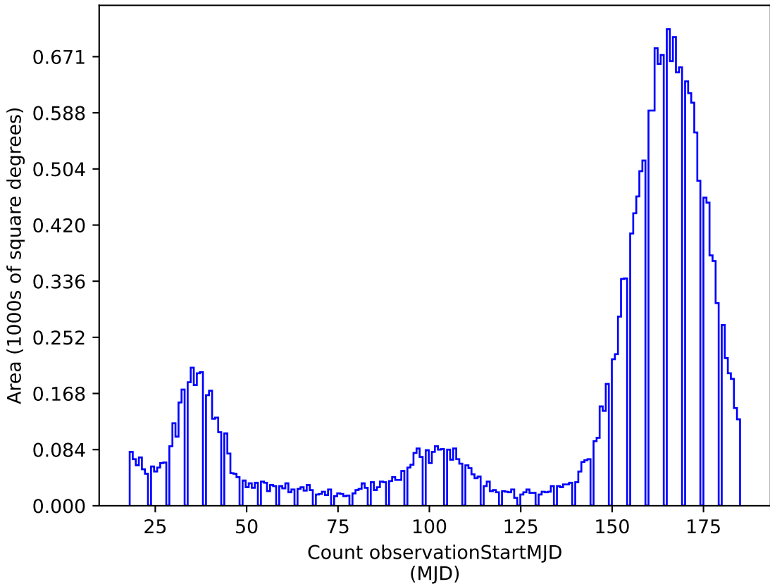
baseline_v3.3_10yrs y: Count observationStartMJD
