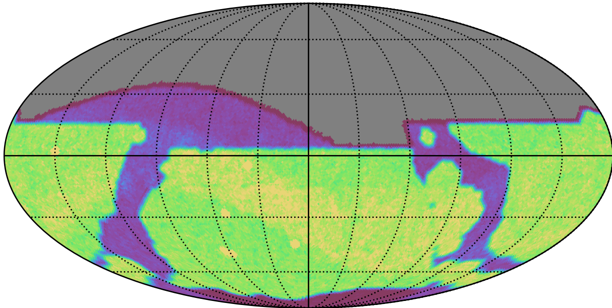
baseline_v3.3_10yrs i: Count observationStartMJD
