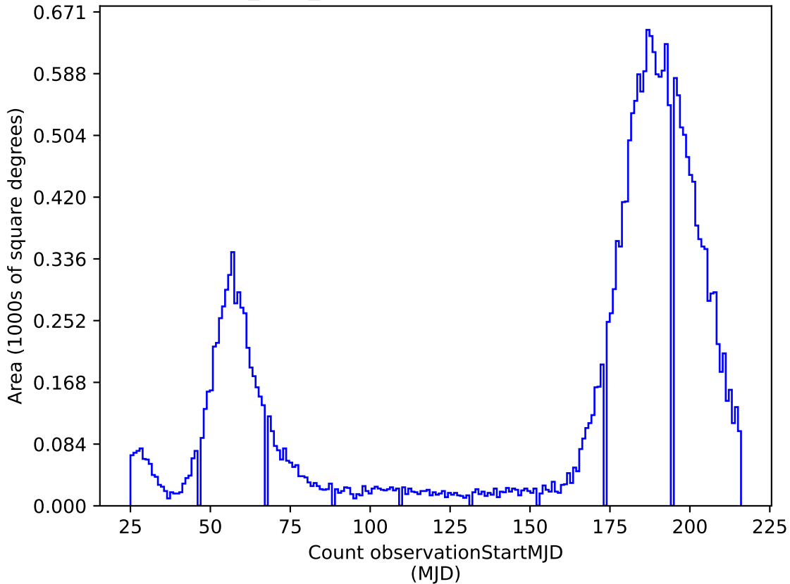
baseline_v3.3_10yrs i: Count observationStartMJD
