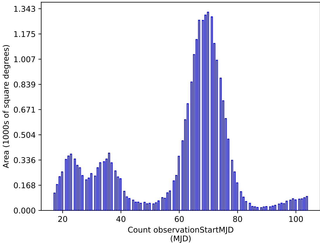
baseline_v3.3_10yrs g: Count observationStartMJD
