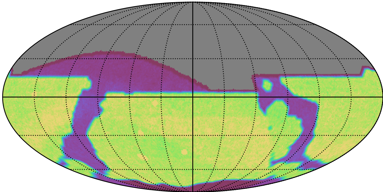
baseline_v3.3_10yrs : Count observationStartMJD
