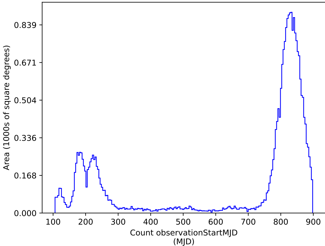
baseline_v3.3_10yrs : Count observationStartMJD
