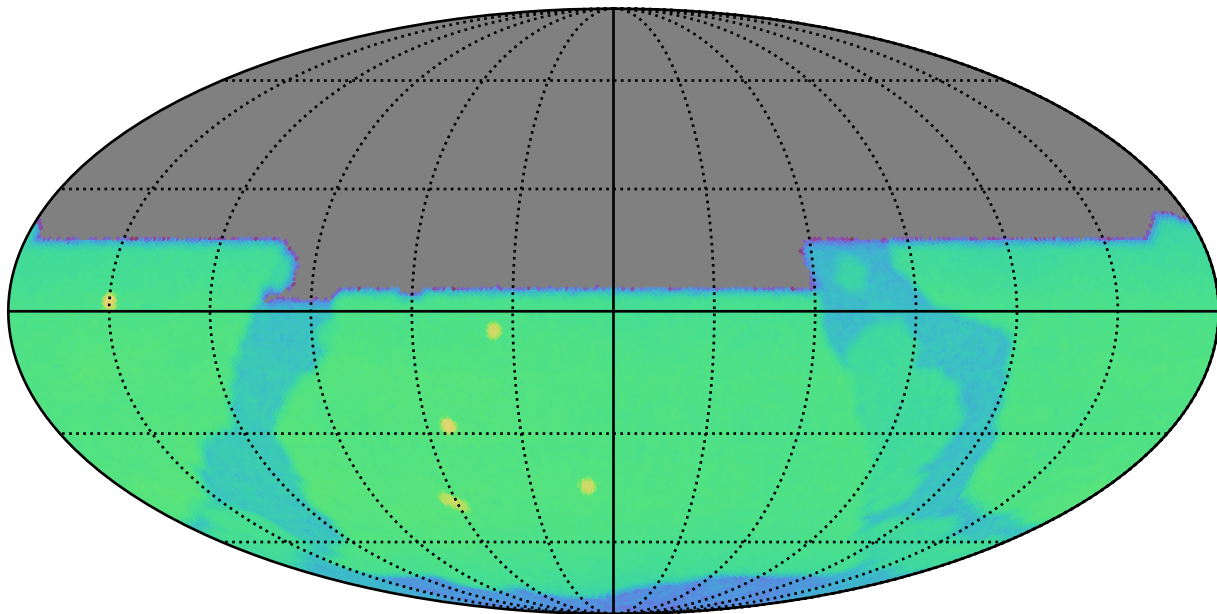
baseline_v3.3_10yrs y: CoaddM5
