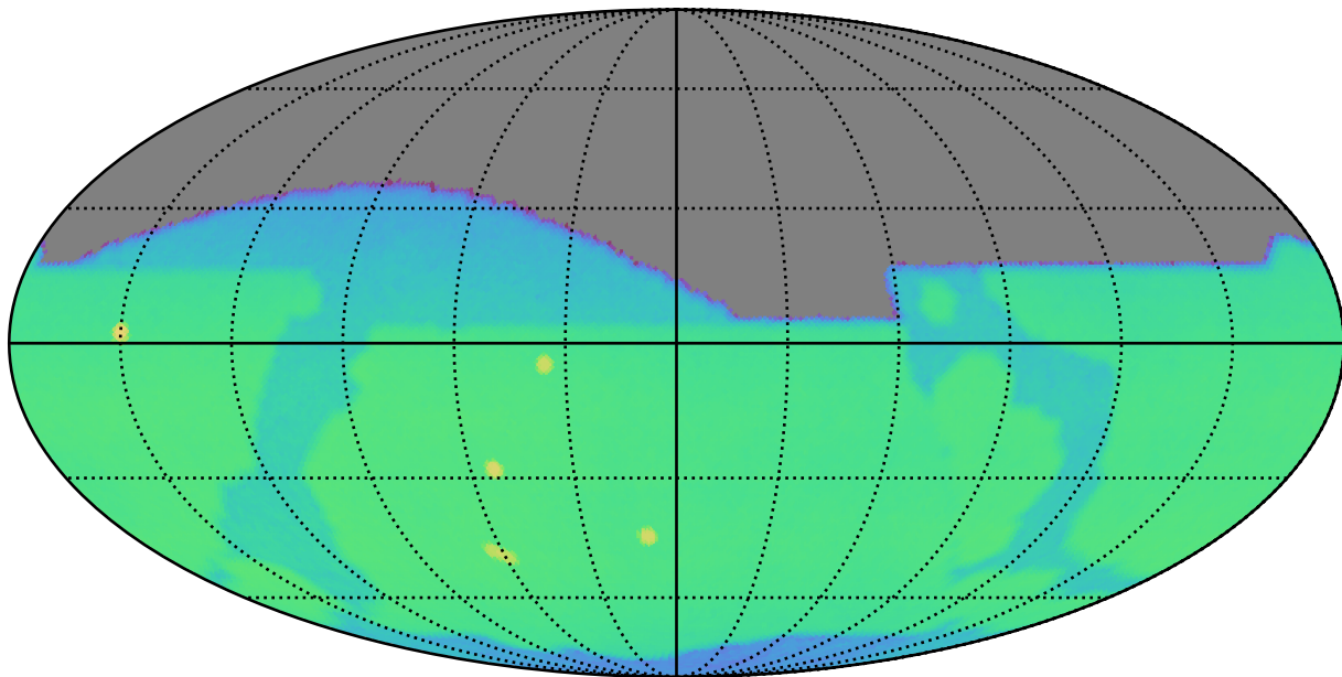
baseline_v3.3_10yrs r: CoaddM5
