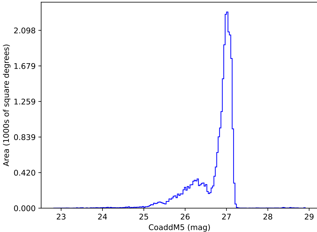
baseline_v3.3_10yrs r: CoaddM5
