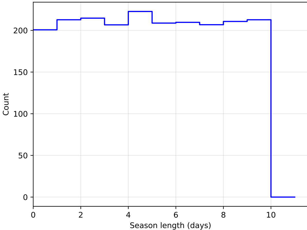
baseline_v3.3_10yrs DD:XMM_LSS all bands: SeasonLength
