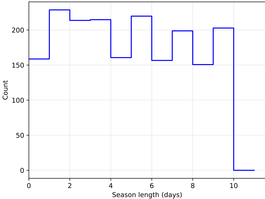
baseline_v3.3_10yrs DD:WFD all bands: SeasonLength
