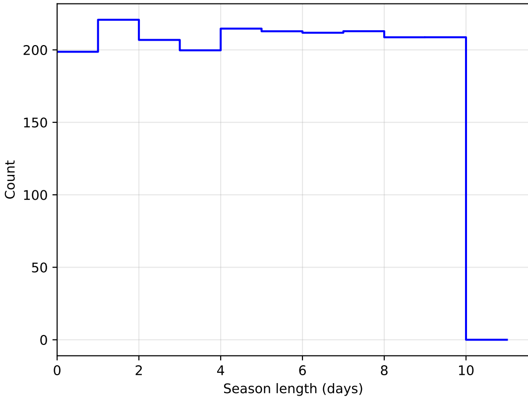
baseline_v3.3_10yrs DD:ELAISS1 all bands: SeasonLength
