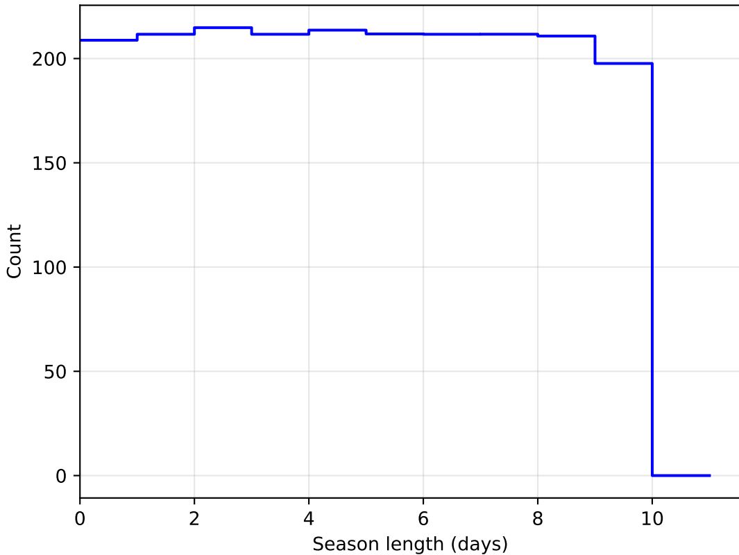
baseline_v3.3_10yrs DD:EDFS all bands: SeasonLength
