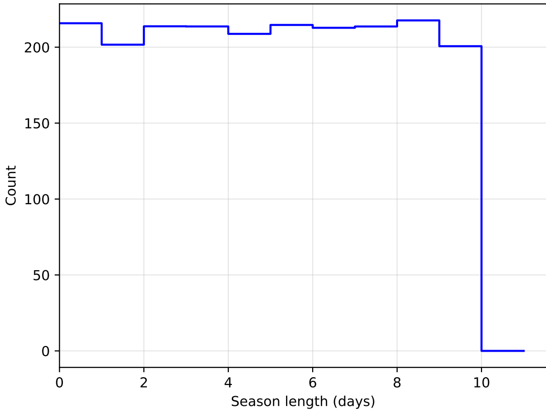
baseline_v3.3_10yrs DD:ECDFS all bands: SeasonLength
