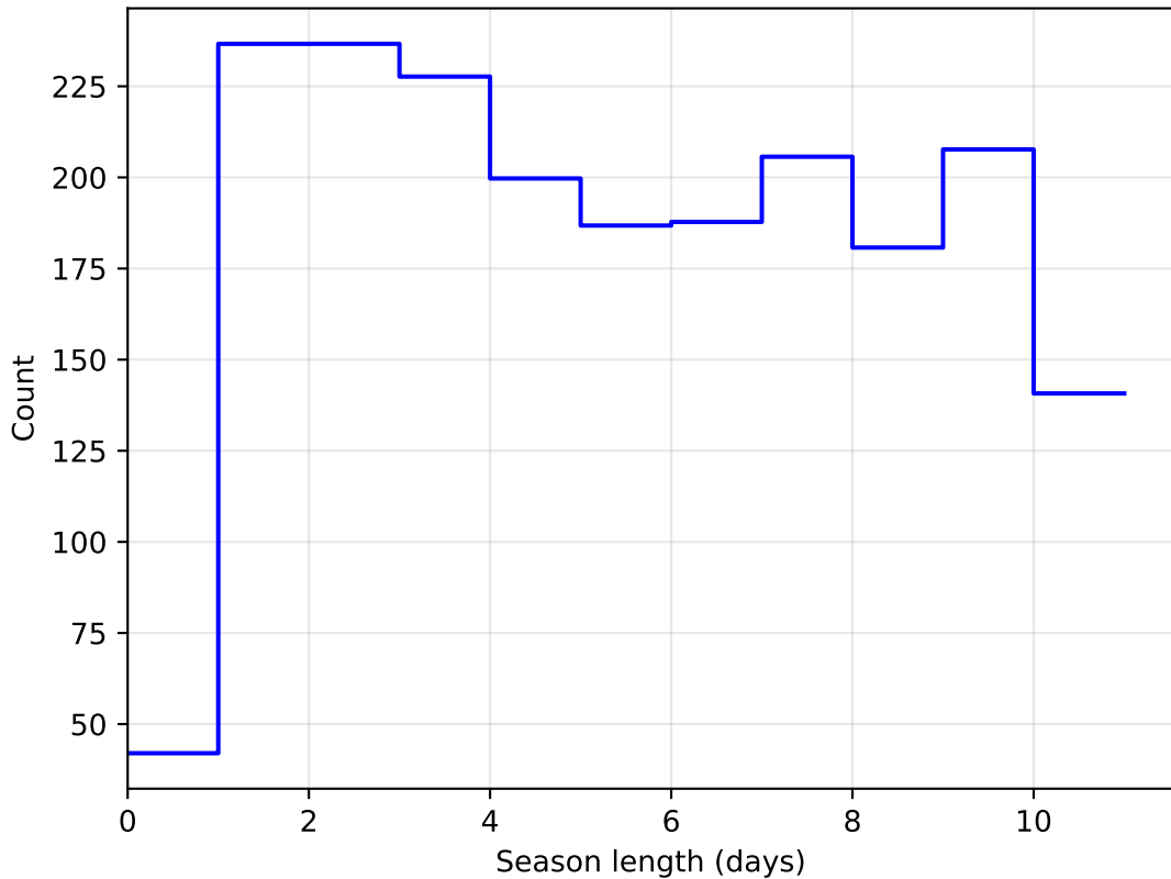
baseline_v3.3_10yrs DD: COSMOS all bands: SeasonLength
