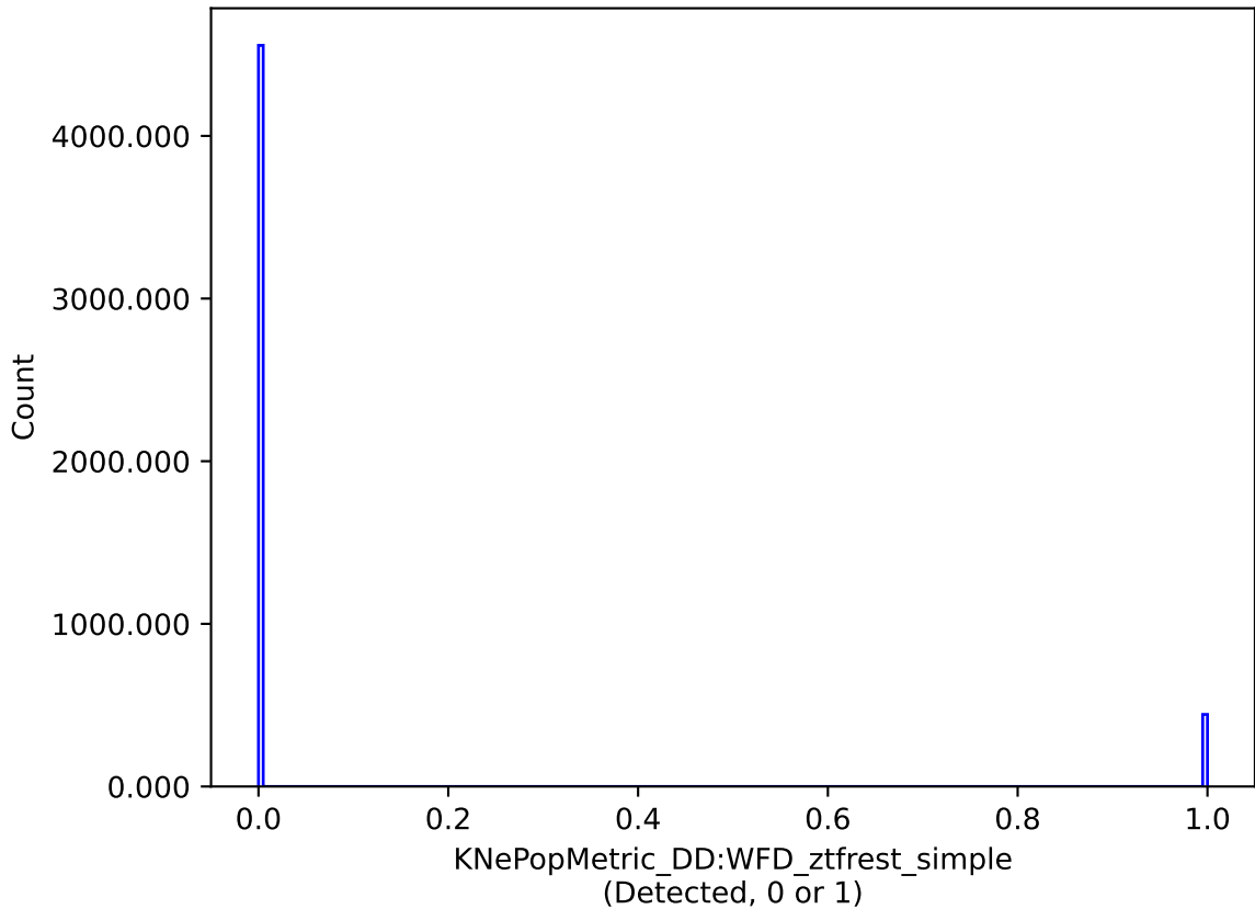
baseline_v3.3_10yrs DD:WFD: KNePopMetric_DD:WFD_ztfrest_simple
