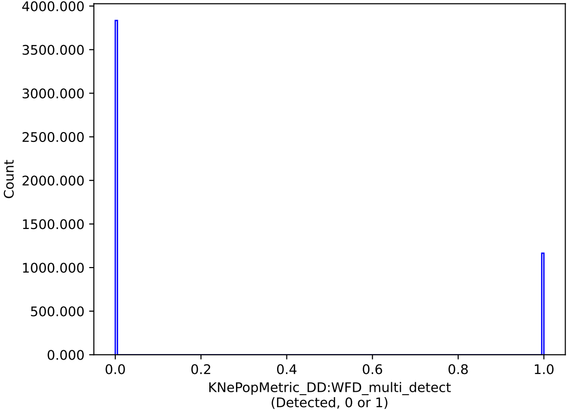
baseline_v3.3_10yrs DD:WFD: KNePopMetric_DD:WFD_multi_detect
