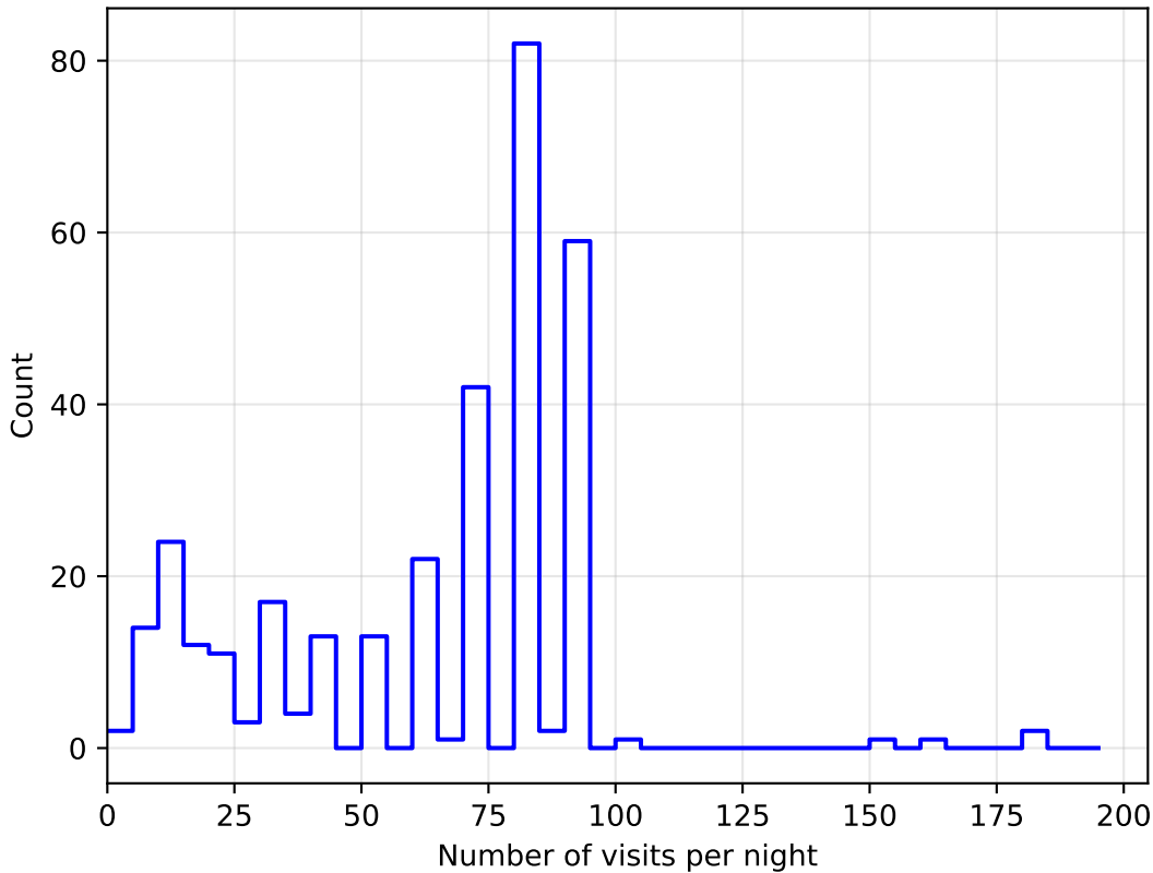
baseline_v3.3_10yrs all bands: DD:XMM_LSS NVisitsPerNight
