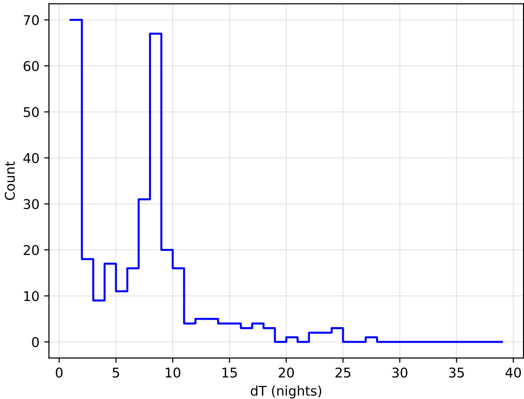
baseline_v3.3_10yrs all bands: DD:XMM_LSS Delta Nights Histogram
