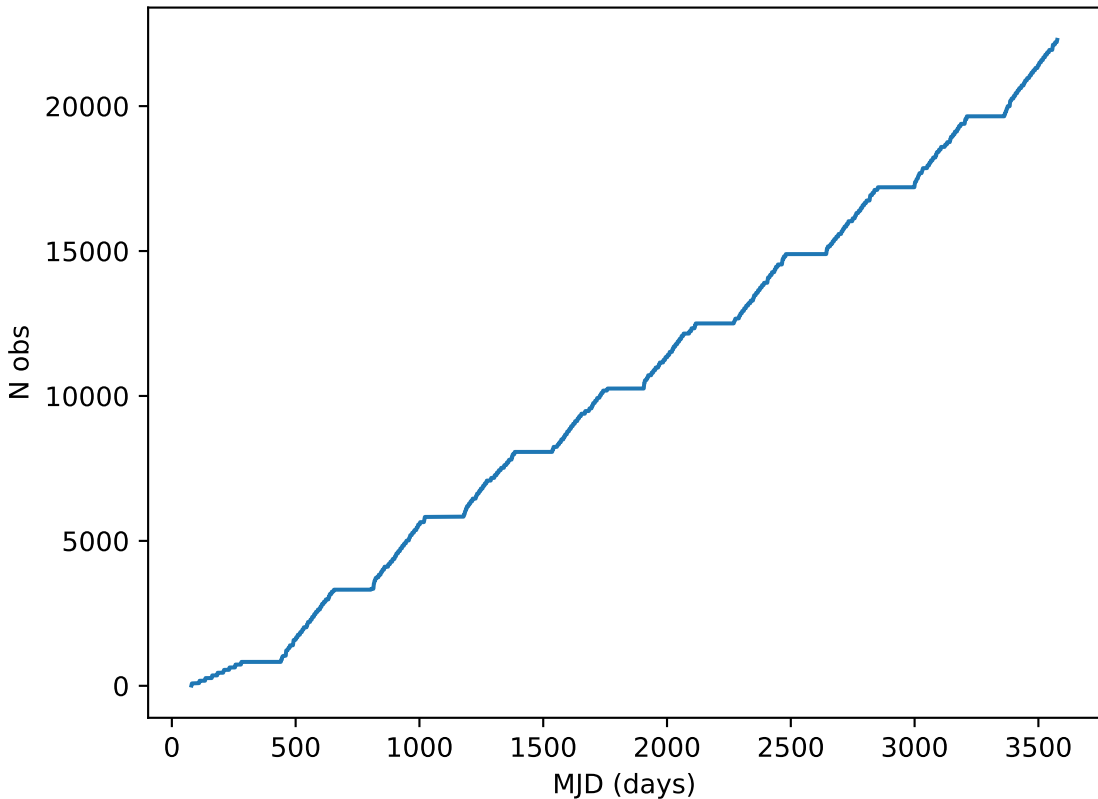
baseline_v3.3_10yrs all bands: DD:XMM_LSS Cumulative NVisits
