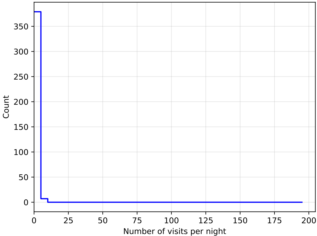
baseline_v3.3_10yrs all bands: DD:WFD NVisitsPerNight
