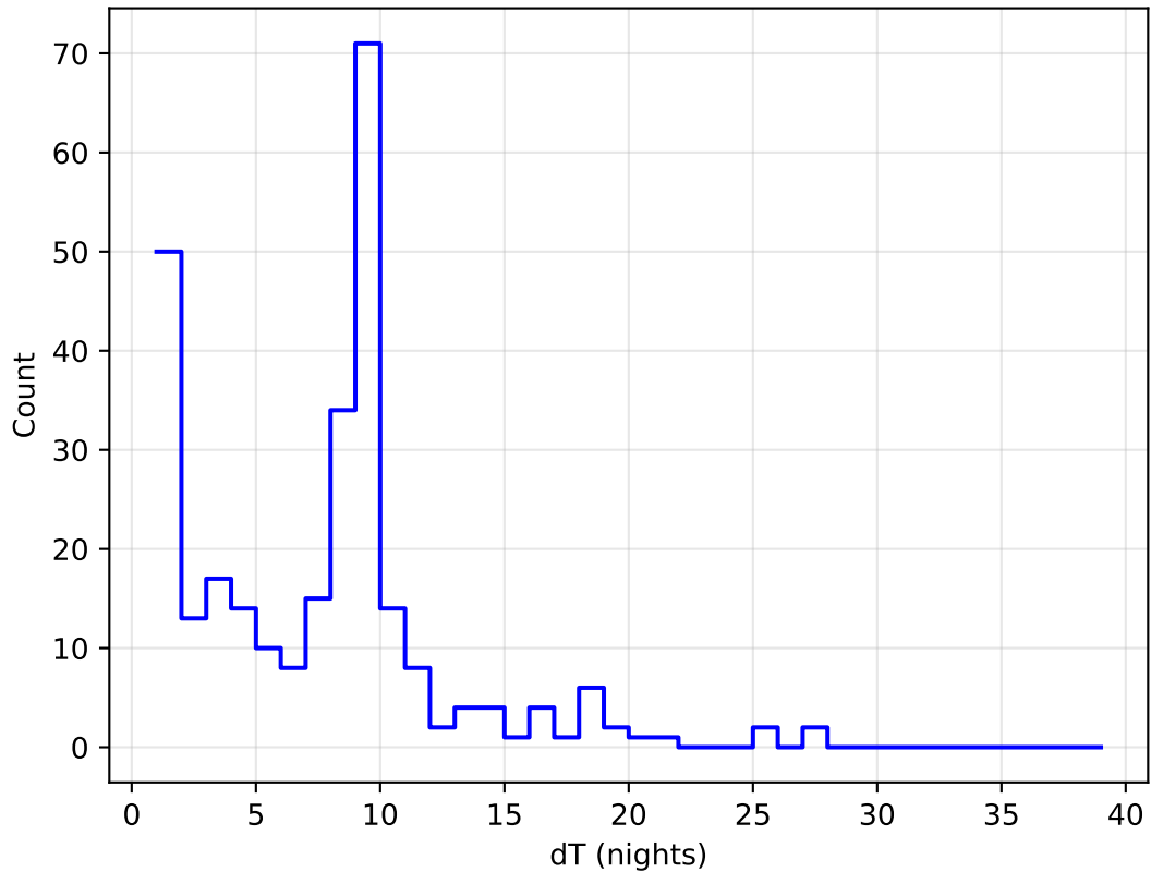
baseline_v3.3_10yrs all bands: DD:ELAISS1 Delta Nights Histogram
