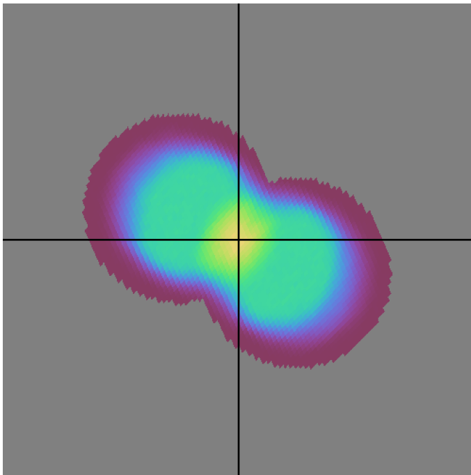
baseline_v3.3_10yrs all bands: DD:EDFS NVisits
