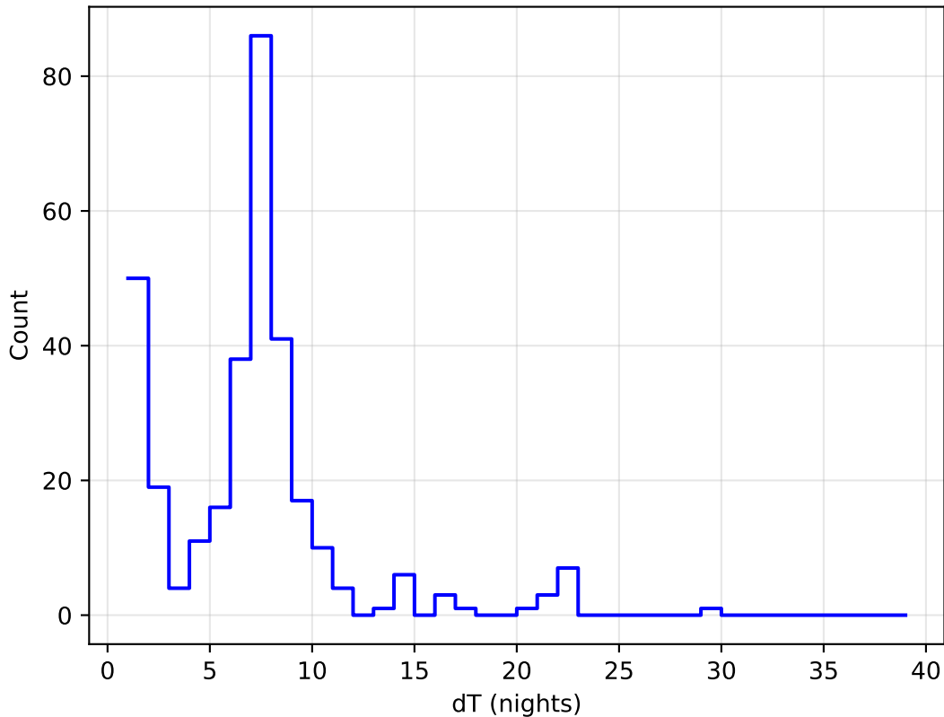
baseline_v3.3_10yrs all bands: DD:EDFS Delta Nights Histogram
