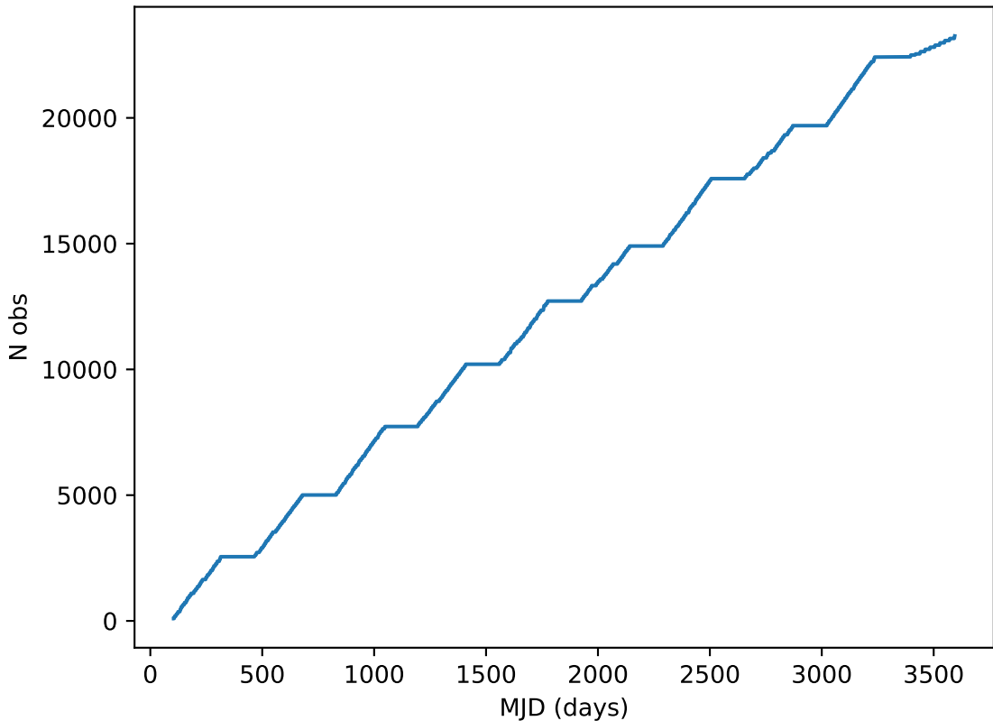
baseline_v3.3_10yrs all bands: DD:EDFS Cumulative NVisits
