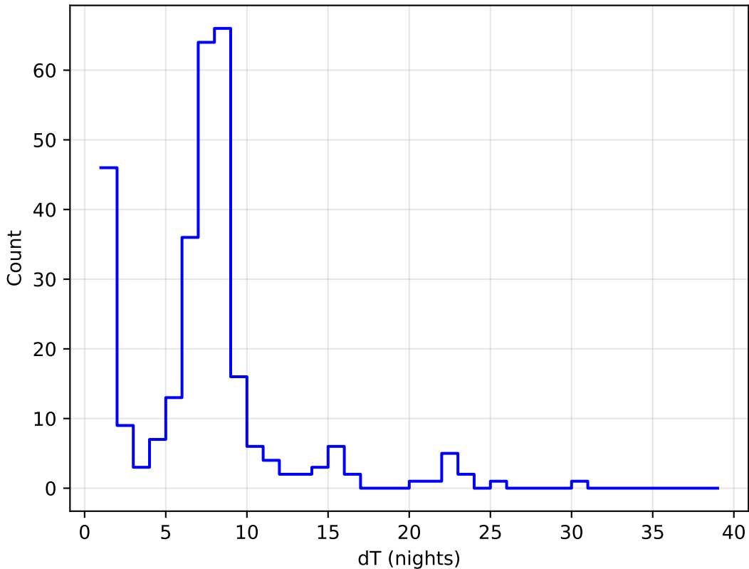
baseline_v3.3_10yrs all bands: DD:ECDFS Delta Nights Histogram
