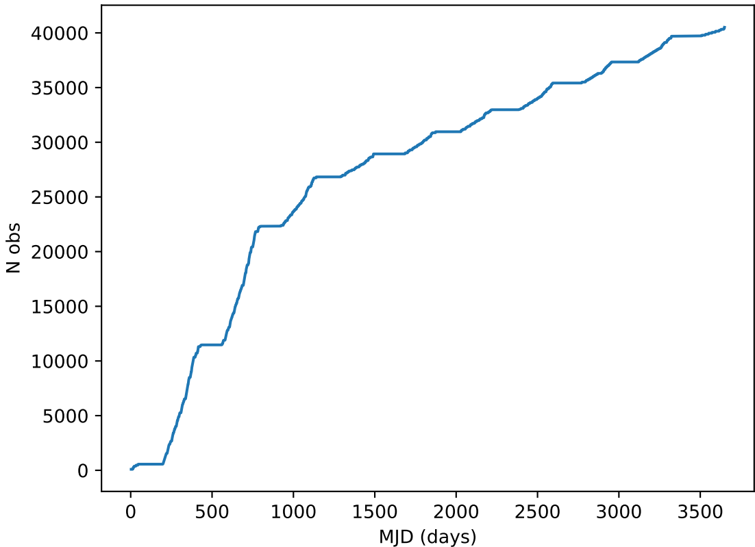
baseline_v3.3_10yrs all bands: DD: COSMOS Cumulative NVisits
