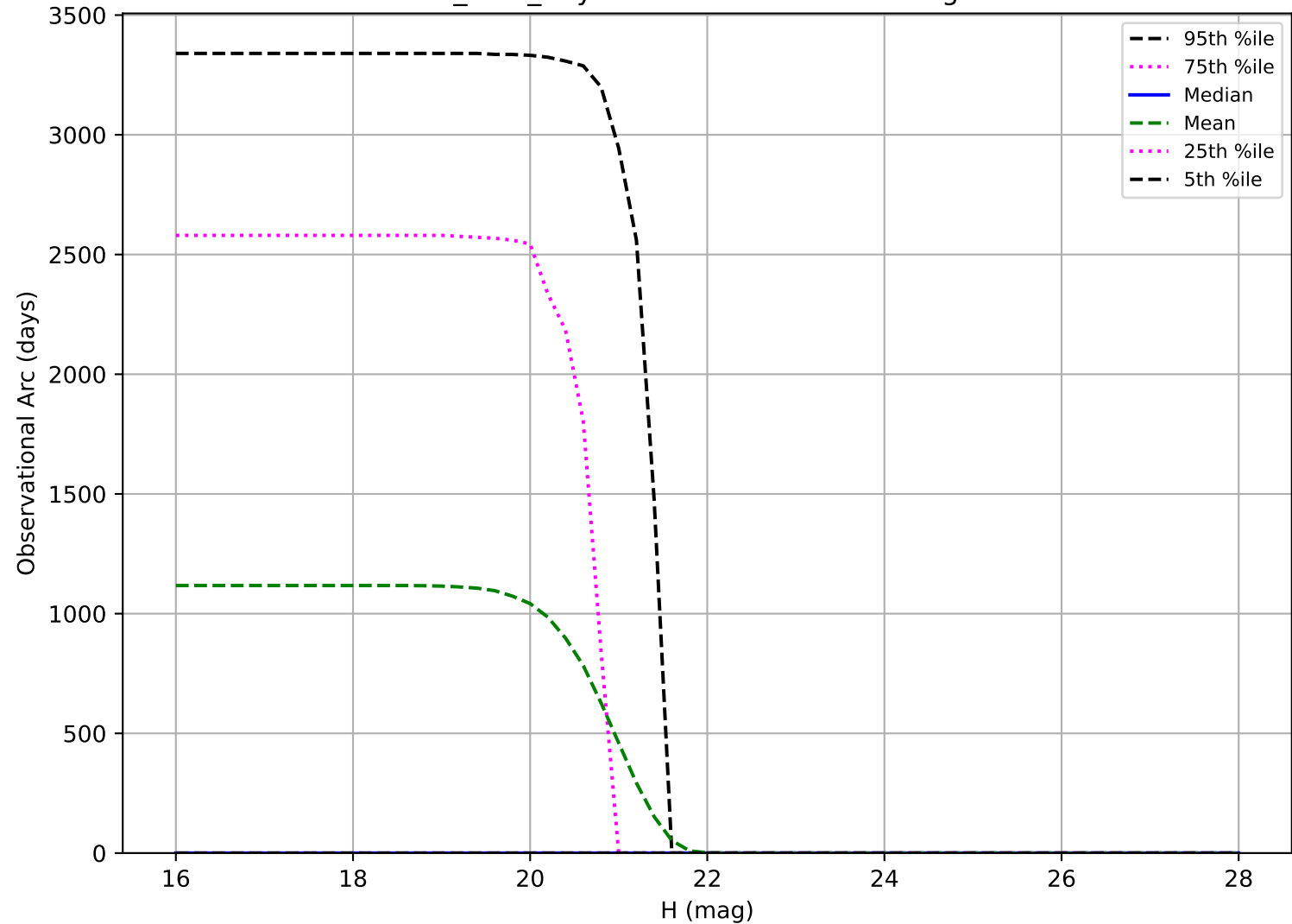
baseline_v3.2_10yrs: Observational Arc Length Vatira
