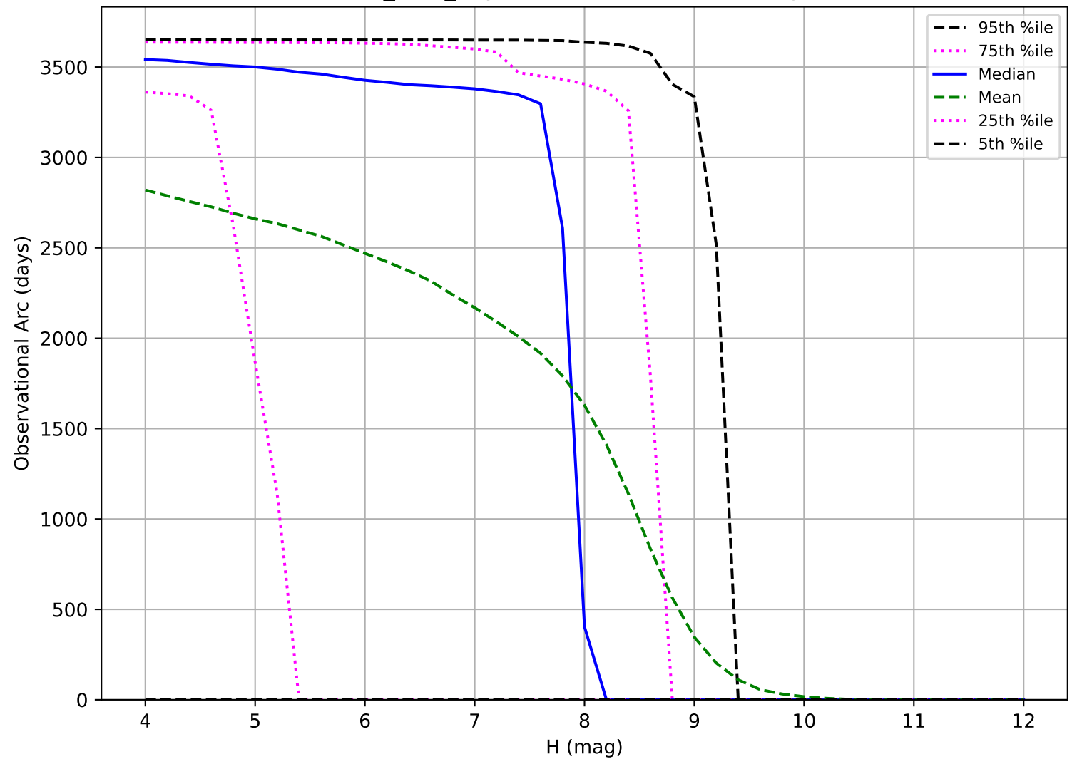
baseline_v3.2_10yrs: Observational Arc Length TNO
