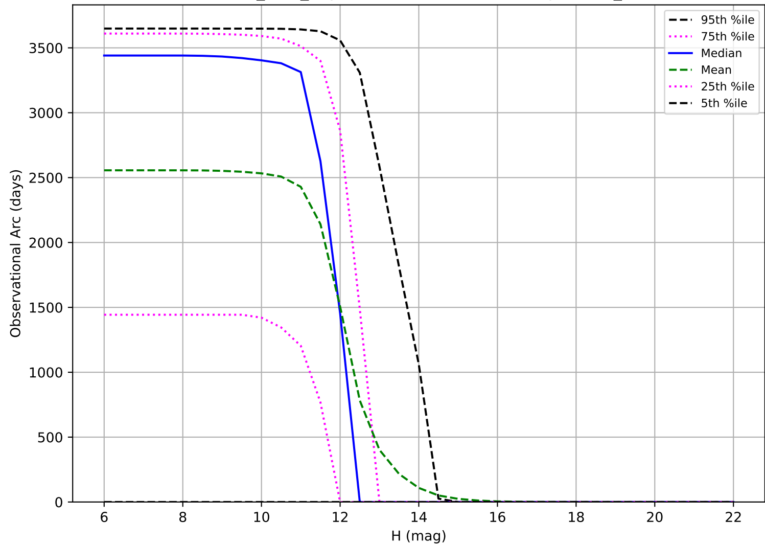
baseline_v3.2_10yrs: Observational Arc Length OCC_r20
