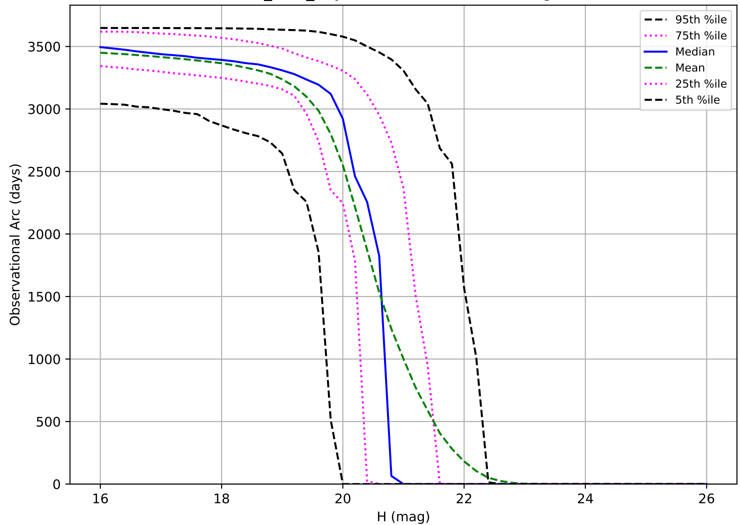
baseline_v3.2_10yrs: Observational Arc Length MBA
