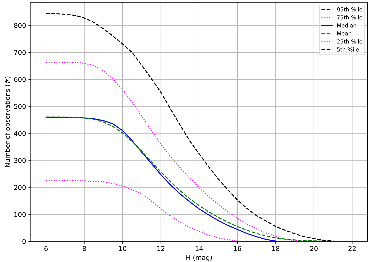
baseline_v3.2_10yrs: Number of observations OCC_r5
