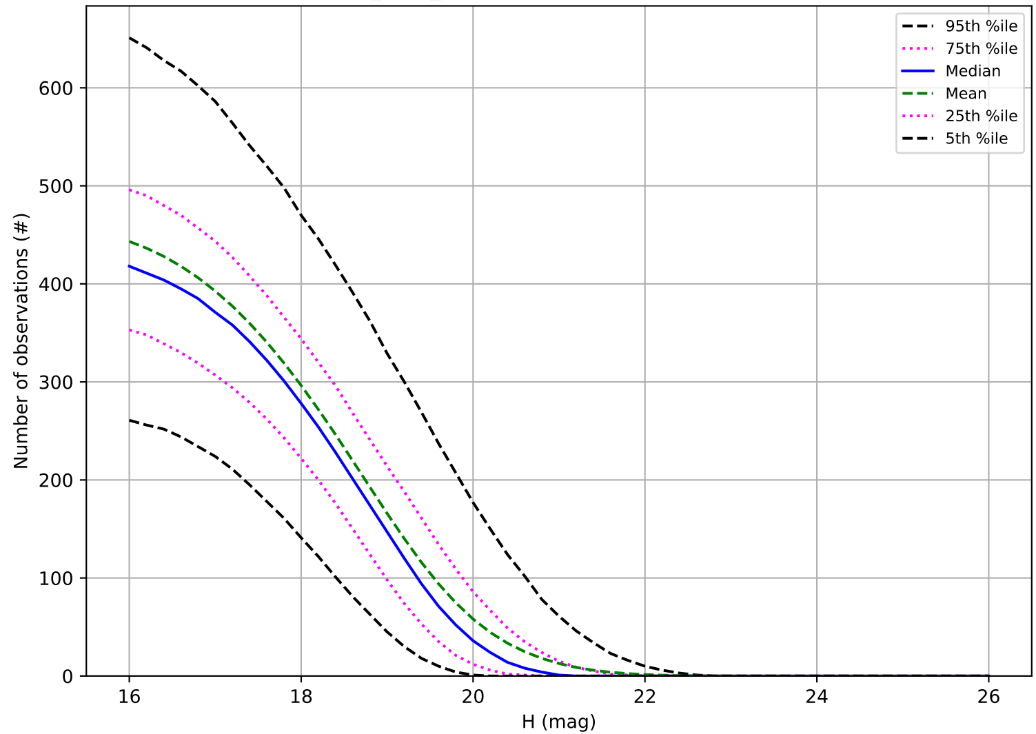
baseline_v3.2_10yrs: Number of observations MBA
