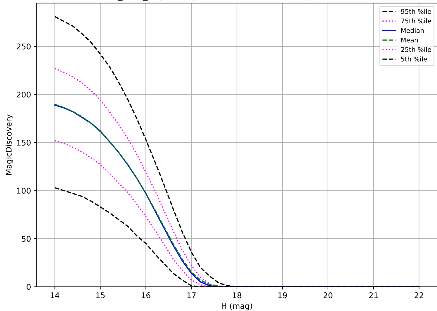
baseline_v3.2_10yrs: Trojan 6 detections in 60 nights detection loss
