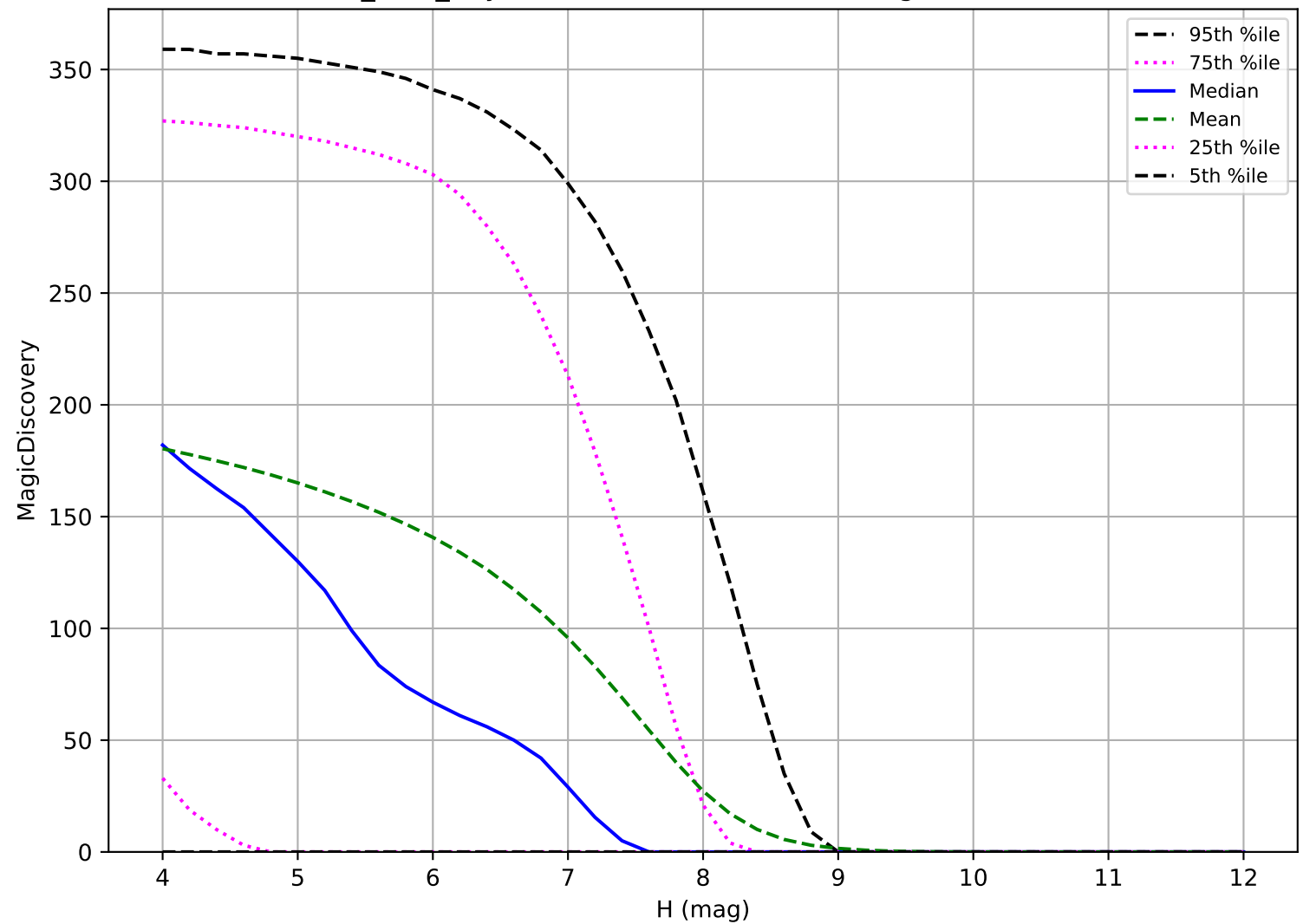
baseline_v3.2_10yrs: TNO 6 detections in 60 nights detection loss
